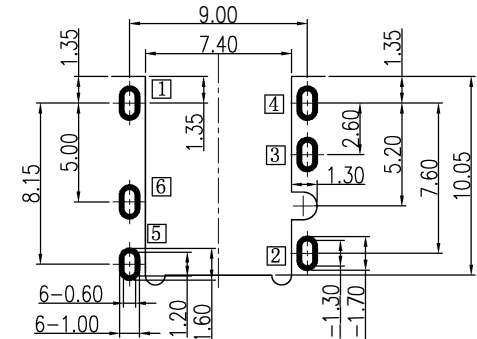
RECOMMENDED P.C.B LAYOUT TOP VIEW (TOLRANCE:±0.05)
